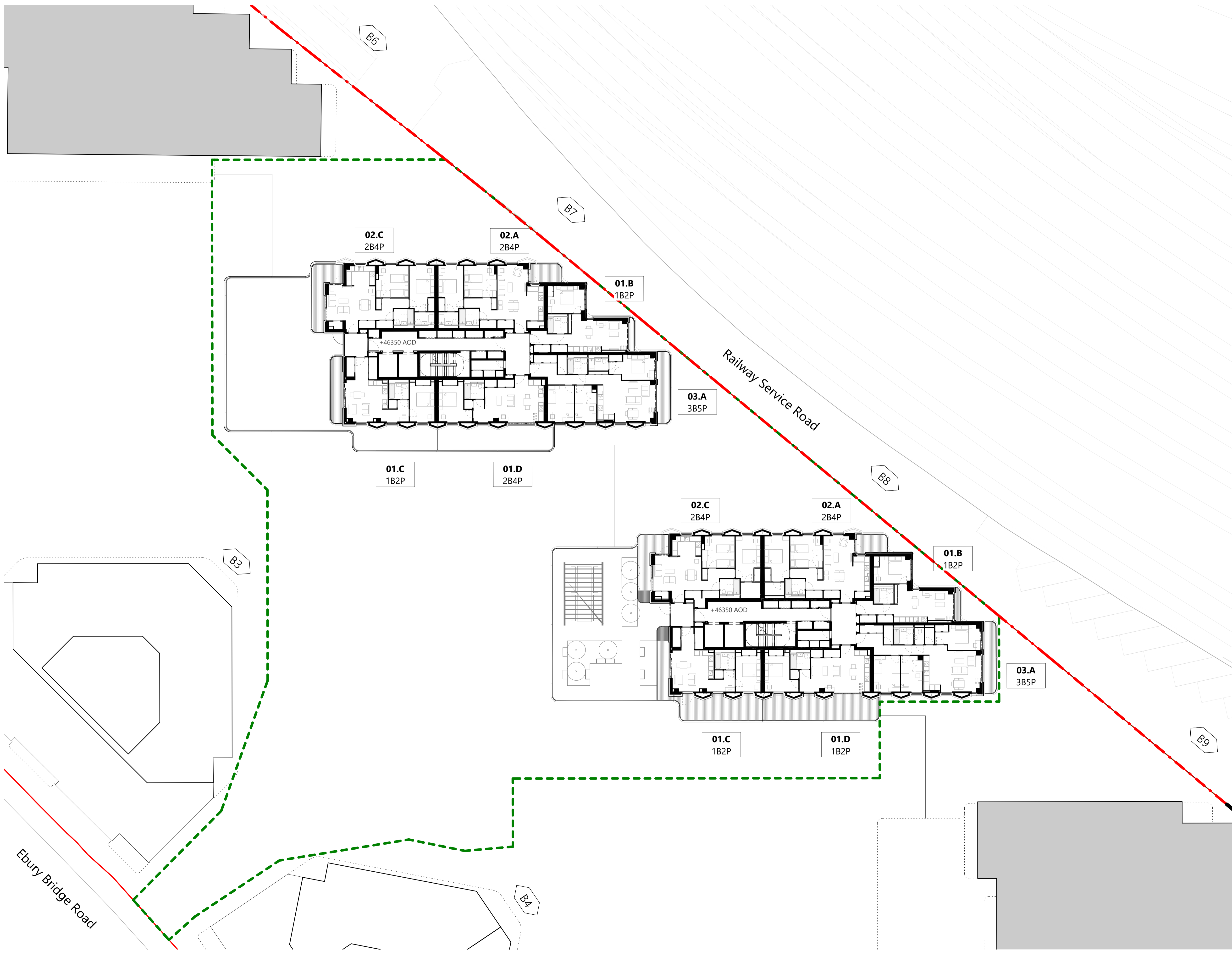
1 Detailed Area-Level 13 1 : 200
