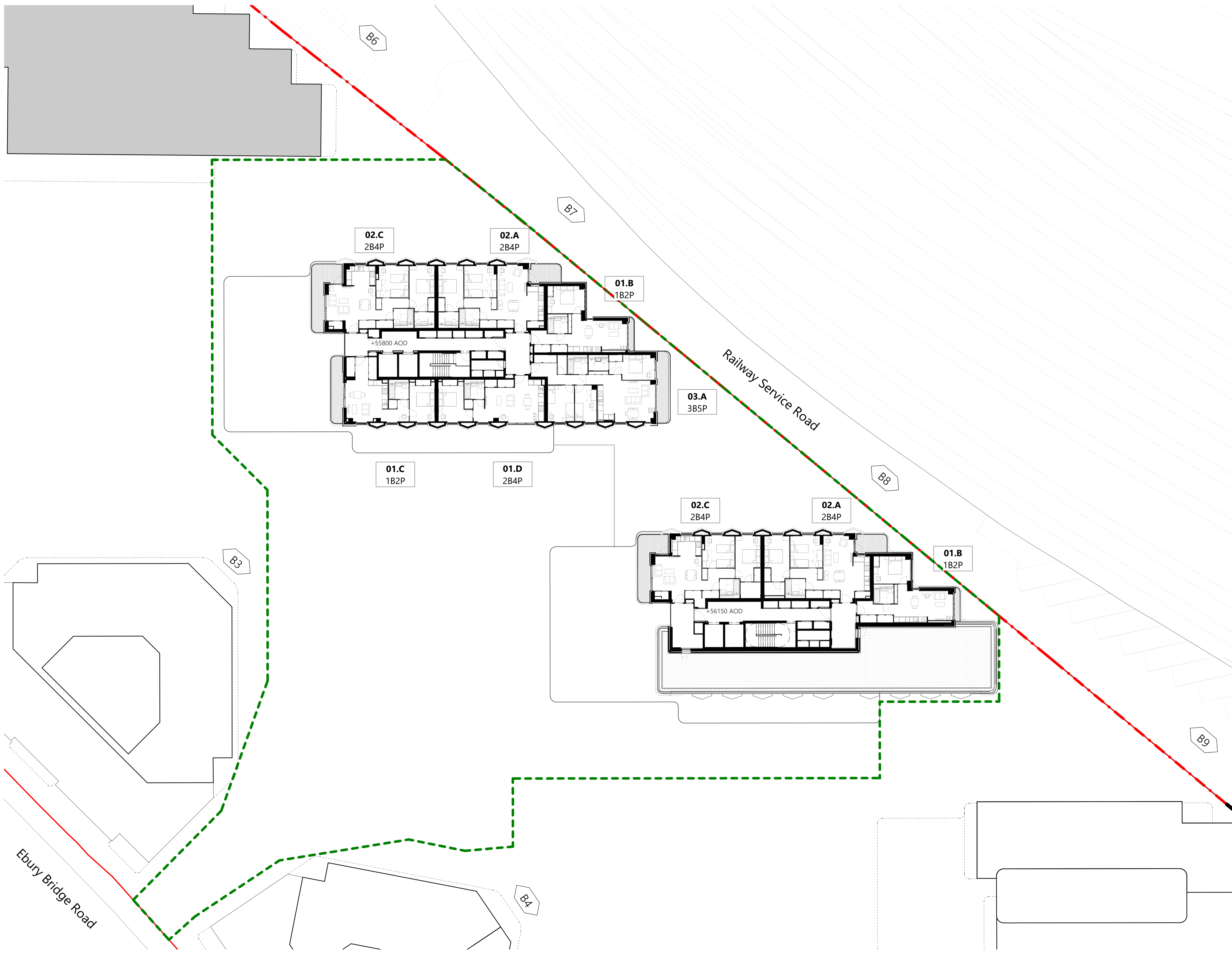
1 Detailed Area-Level 16 1:200
