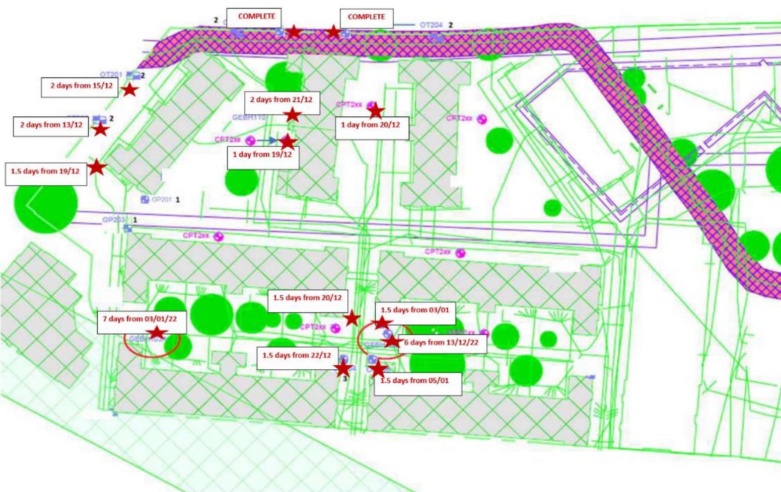
Map of Phase 2 showing the location of each borehole and how long each hole is expected to take to dig.
